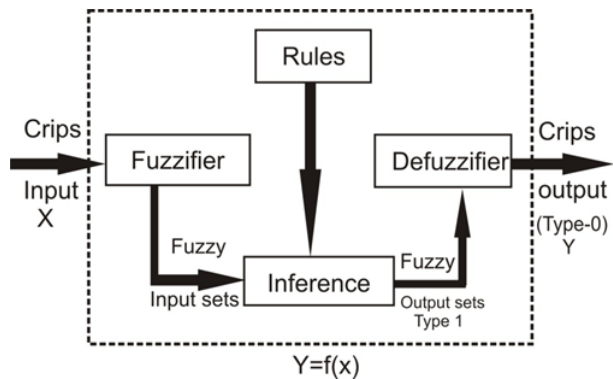
Figure 1. Fuzzy System.
