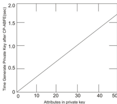
Figure 2. Key Generating Time.
