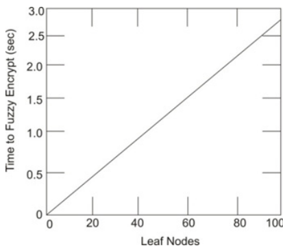
Figure 3. Fuzzy encryption time.
