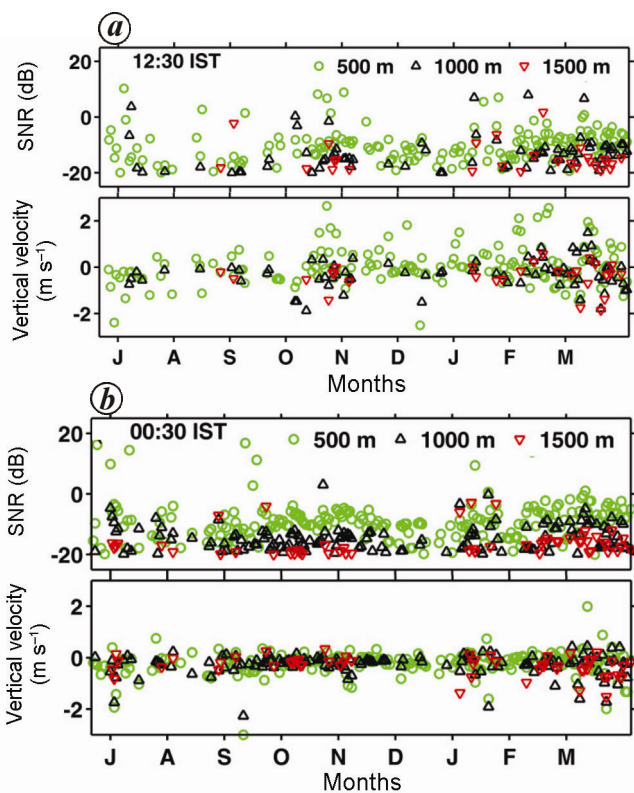
Figure 4. Time series of daily mean SNR and vertical velocity ( \text{m s}^{-1} ) ( a ) during strong convective period during daytime 07 : 00 UT (12 : 30 IST) and ( b ) for the stable conditions around midnight 19 : 00 UT (00 : 30 IST). The convective updrafts are stronger during daytime and at lower altitudes. The magnitudes of updrafts are the least during the rainy monsoon months and start increasing from November reaching their peak values by March.
