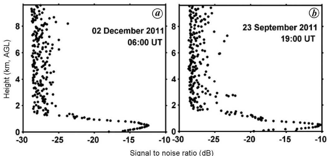
Figure 3. Vertical profiles of DL signal-to-noise ratio (SNR). a , For a typical convective condition on 2 December 2011 at 06 : 00 UT (11 : 30 IST); b , For the nocturnal stable condition on 23 September 2011 at 19 : 00 UT (00 : 30 IST). We have observed the less noisy data up to 2 km, AGL over the site in both convective and stable atmosphere.
