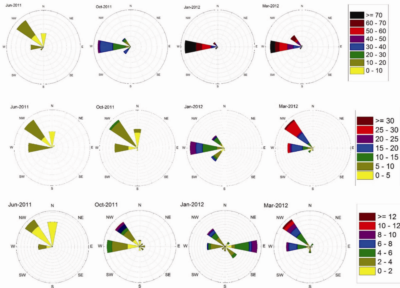
Figure 3. Wind rose plots at 2, 5 and 10 km (bottom to top) altitude during June 2011, October 2011, January 2012 and March 2012 at ARIES, Nainital.
