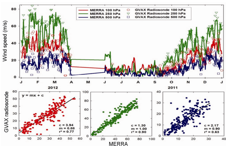
Figure 6. Monthly variations in observed and MERRA wind speed at peak altitude of subtropical jet, i.e. 250 hPa, and also at 100 and 500 hPa. Correlation between them in the three altitude regions is also shown.
