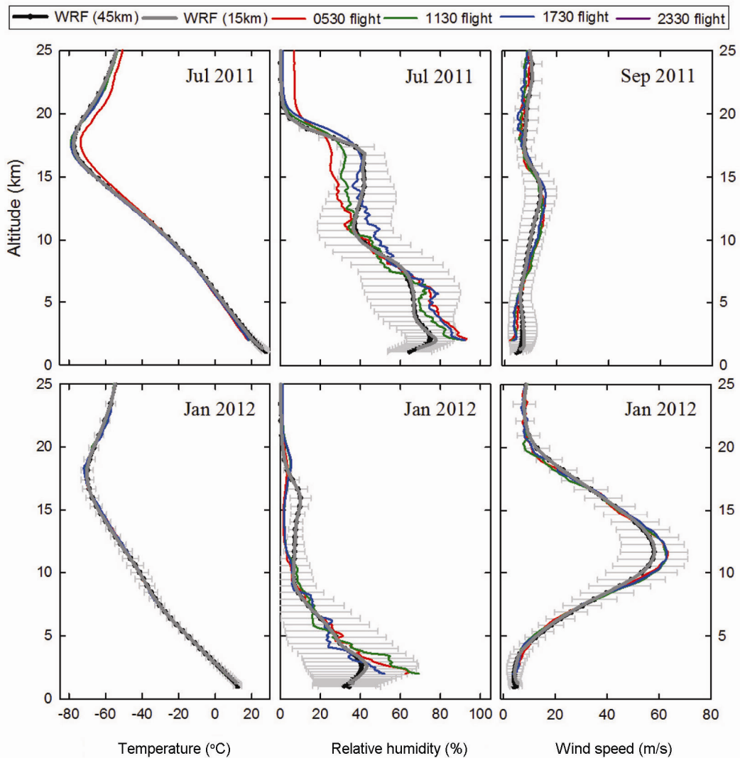
Figure 5. Vertical distribution of temperature, relative humidity and wind speed from radiosonde observations and WRF model simulations during winter (January 2012) and summer monsoon (July 2011). Wind speed is not available for July and is shown for September 2011.
