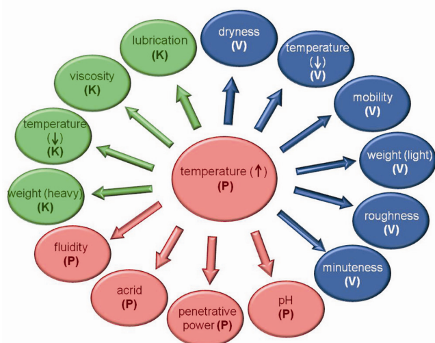
Figure 2. An illustrative example of intra- and inter-connections between parameters of Vata (V), Pitta (P) and Kapha (K). The associations between a factor of P (temperature) with its co-factors, and those of V and K are shown. (↑, Increase; ↓, Decrease).
