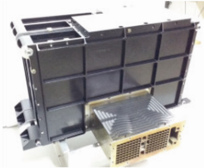
Figure 4. Engineering model of the HELIOS payload.
