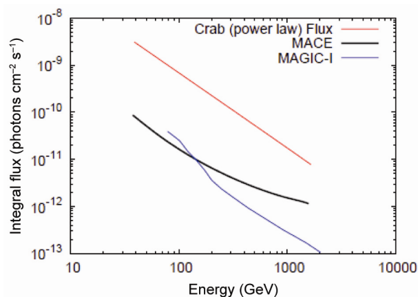
Figure 1. Comparison of the integral sensitivity of the MACE and the MAGIC-I telescopes at 5° zenith angle. The Crab Nebula power law spectrum is also plotted for reference.
