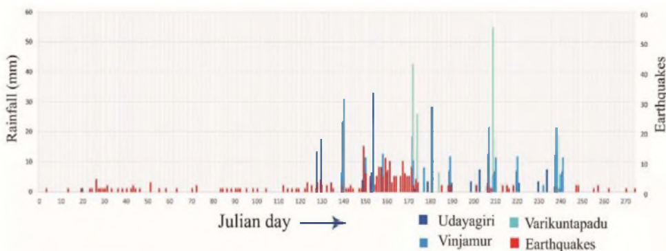
Figure 3. Histogram showing rainfall data versus number of earthquakes per day located in the study region.
