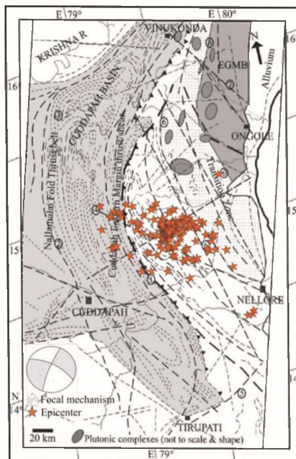
Figure 1. Plot of epicentres on image interpretation of landsat TM 11 . Some of the major lineaments (shown with numbers) are: (1) Cuddapah Boundary Thrust, (2) Nallamalai/Rudravaram Line, (3) Gani-Kalva Fault, (4) Nellore-Badvel Fault, (5) Karakambadi Fault, (6) Terrane Boundary Shear Zone (TBSZ) and (7) Gundlakamma Fault.
