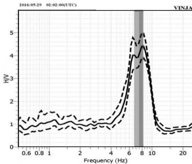
Figure 2. H/V spectral ratio plot for ambient noise recorded at Vinjamur Seismic Station.
