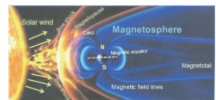
Magnetosphere of the Earth
