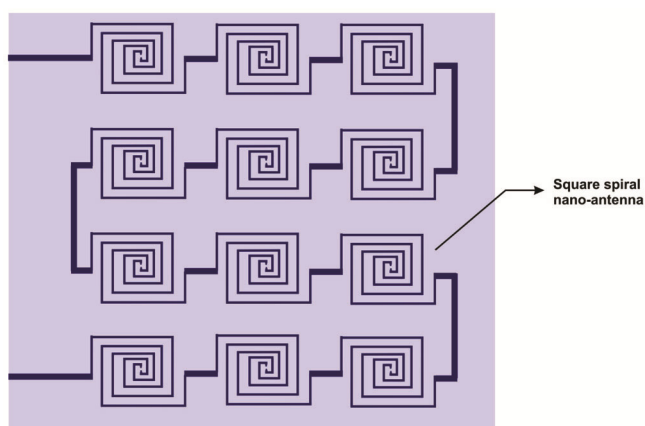
Figure 4. An array of square spiral nano-antennas.
