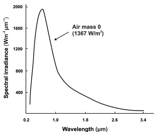
Figure 2. Spectral irradiance for air mass in outer space (AM0) which resembles the blackbody radiation spectrum.
