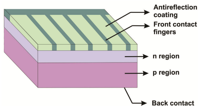
Figure 3. Basic structure of a p–n junction solar cell.
