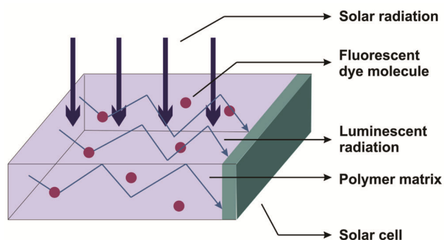
Figure 5. Guidance of luminescent radiation in luminescent solar concentrator by total internal reflection.
