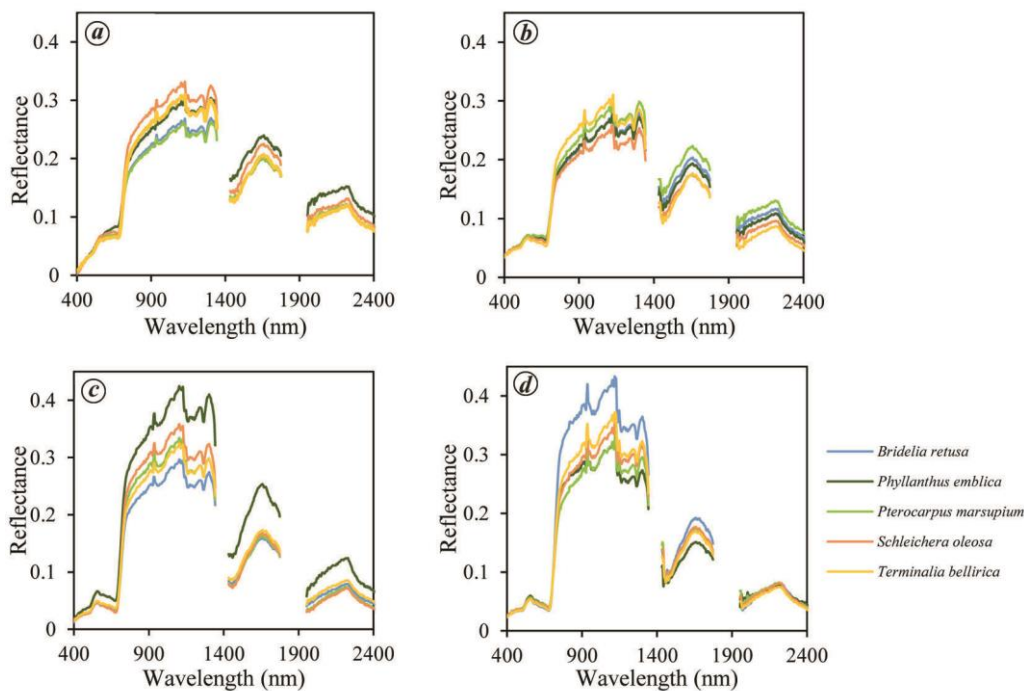
Figure 1. Mean canopy spectra ( n = 2-50 ) of 5 of the 16 common species showing inter-species spectral variability: a , Shoolpaneshwar Wildlife Sanctuary (SWS); b , Vandsa National Park (VNP); c , Mudumalai Tiger Reserve (MTR); d , Sholayar Reserve Forest (SRF).
