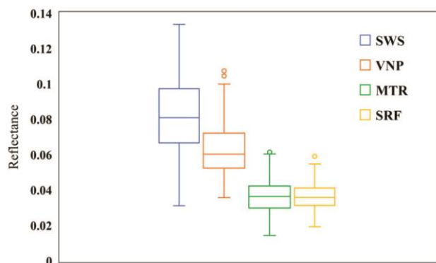
Figure 4. Boxplots ( n = 200 , from spectra of 16 common species) developed from reflectance values at 676.96 nm.
