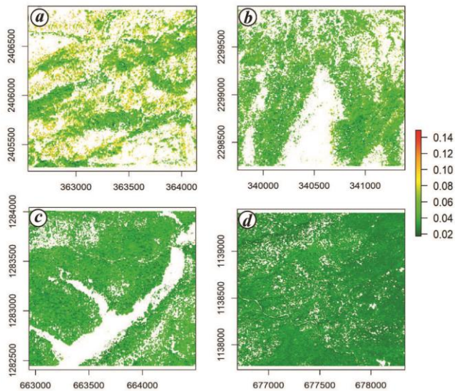
Figure 3. Map of reflectance measured at chlorophyll absorption band (676.96 nm) showing phenology phase variations in the four forest covers: a , SWS; b , VNP; c , MTR; d , SRF.
