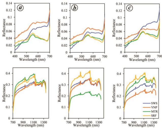
Figure 2. Intra-species spectral variability over the four forest covers in the spectral region 400–700 and 700–1400 nm: a , Albizia odoratis-sima ; b , Albizia saman ; c , Tectona grandis .
