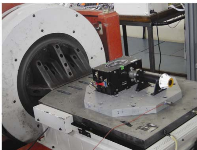
Figure 6. Vibration test set-up for the qualification model of MENCA.
