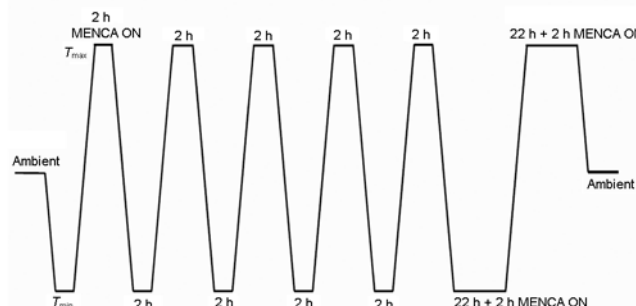
Figure 7. Temperature profile of the thermovacuum test undergone by MENCA. The temperature limits are T_{\min} = +5^{\circ}\text{C} and T_{\max} = +45^{\circ}\text{C} .
