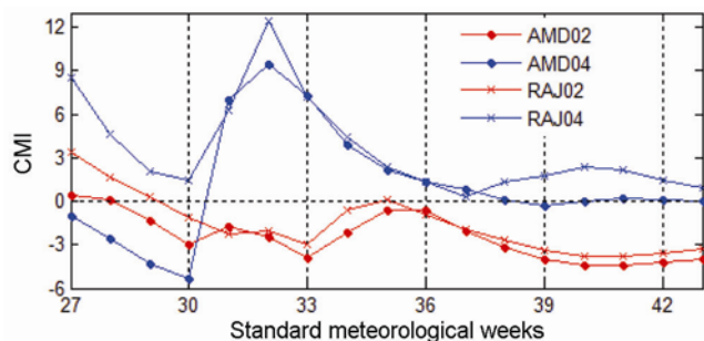
Figure 2. CMI plotted for the meteorological standard week between 27 and 43 weeks (i.e. 2 July to 28 October) representing kharif season (rainy season). Week nos 35–43 (i.e. early September to end of October) indicate late stage of the crop. AMD and RAJ represent two meteorological stations located at Ahmedabad and Rajkot respectively. CMI plotted for the year 2002 (red line) and 2004 (blue line).
