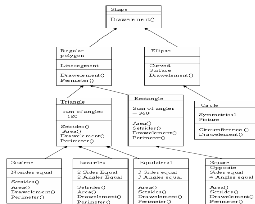
Figure 3: Types of Shapes Using Class Inheritance
