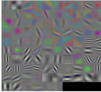
Figure 4. Filters learned on the first layer of CNN (Alex-Net) on IIT Iris Database
