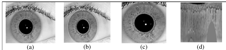
Figure 3. The result of segmentation and normalization stage for (Image 01-L) from IIT Iris Database (a) Original input image. (b) Detected iris and pupil boundary. (c) segmented iris image. (d) Normalized iris image.
