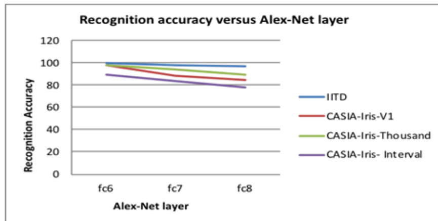
Figure 6. The recognition accuracy after segmentation stage versus different Alex-Net layer
