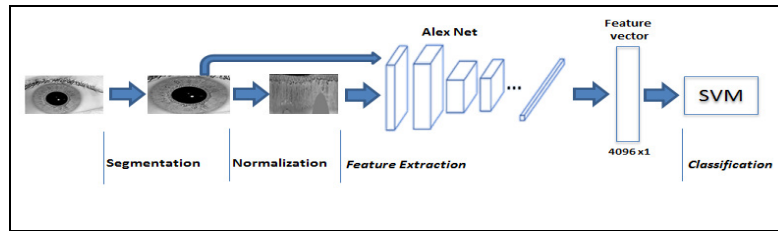
Figure 1. The proposed iris recognition system using Convolutional Neural Network (Alex Net) for feature extraction
