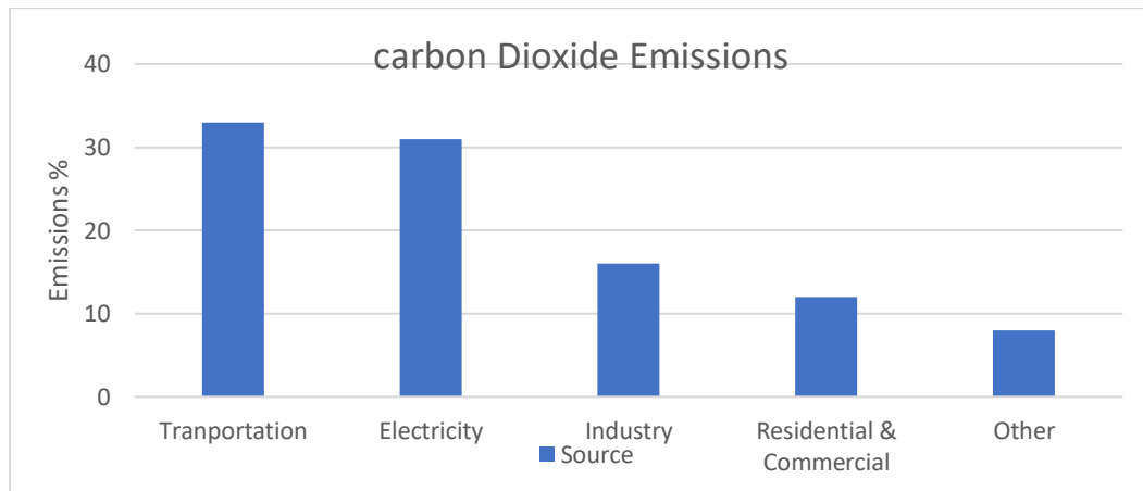
Source: Factors contributing to CO 2 emission [2]
