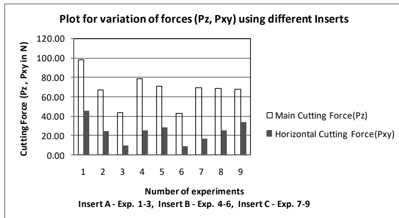
Fig. 2 Plot of change in average forces ( P_z , P_{xy} ) using different Inserts (Insert-A, Insert-B & Insert-C) for set I.
