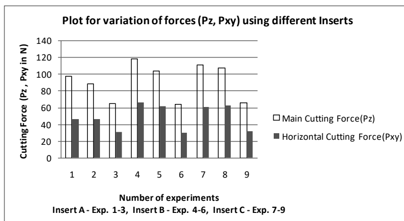
Fig. 4 Plot of change in average forces ( P_z , P_{xy} ) using different Inserts (Insert-A, Insert-B & Insert-C) for Set II
