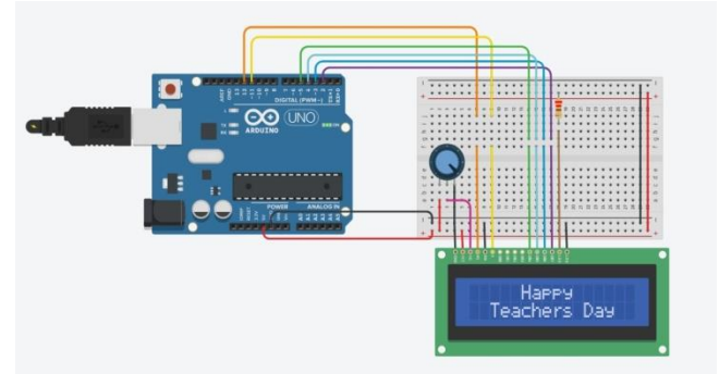
Fig 1: Sample Arduino Circuit created by students to wish all the teachers on Teacher’s day Virtual celebrations
