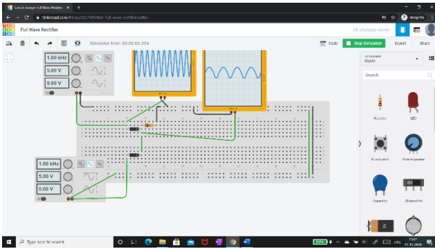
Fig 7: Circuit of Full Wave Rectifier in Tinkercad after simulation with output waveform
