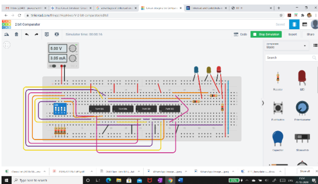
Fig 8: Circuit of a 2 bit comparator using logic gates in Tinkercad
