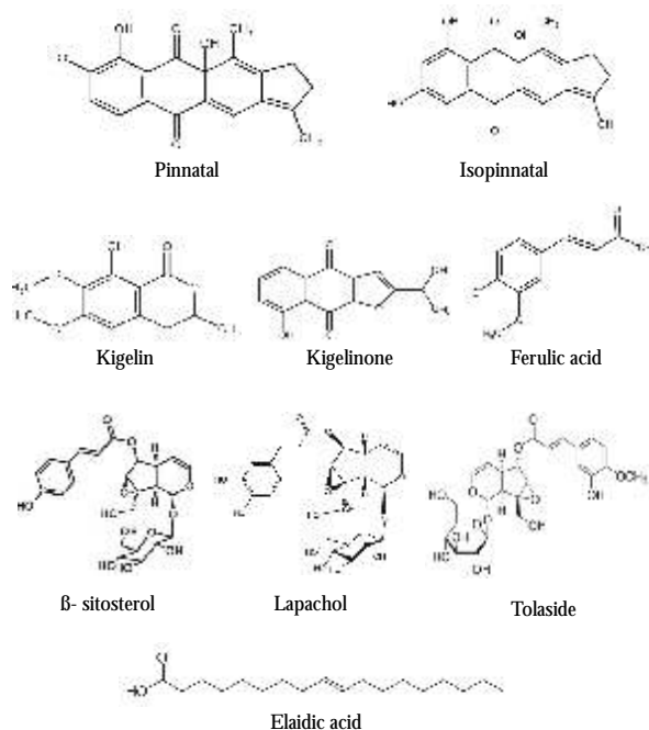
Fig. 4: Chemical constituents present in Kigelia pinnata
