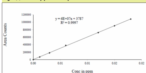
Fig. 3(c): Linearty plot Glimepiride
