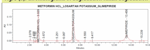
Fig. 5 (b): chromatograms of degradation-Alkali degradation
