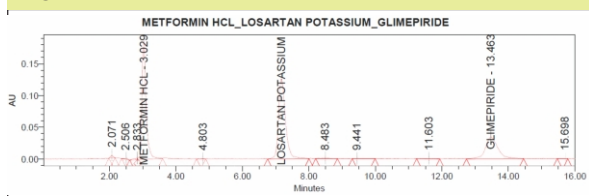
Fig. 5 (c): chromatograms of degradation- of peroxide degradation
