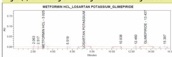
Fig. 5 (a): chromatograms of degradation- acid degradation
