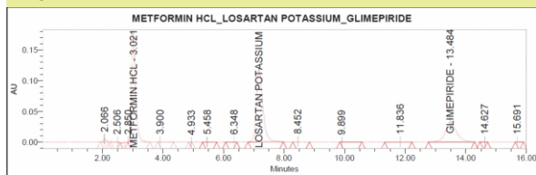
Fig. 5 (f): chromatograms of degradation- thermal degradation
