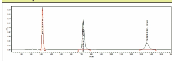
Fig. 2: Typical Chromatogram of Metformin, Losartan and Glimepiride
