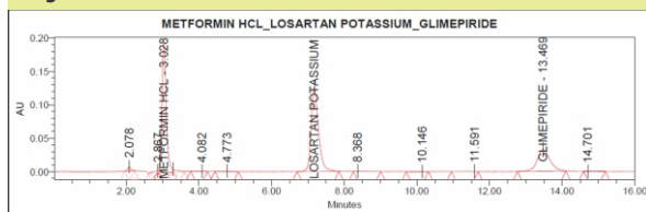
Fig. 5 (g): chromatograms of degradation- Photolytic degradation
