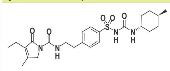
Fig. 1(c): Structure of Glimepiride
