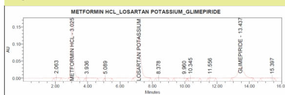
Fig. 5 (e): chromatograms of degradation - Hydrolysis degradation
