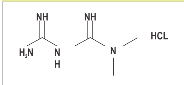
Fig. 1(a): Structure of Metformin
