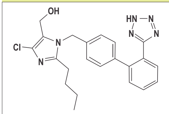
Fig. 1(b): Structure of HCL Losartan (c) Glimepiride
