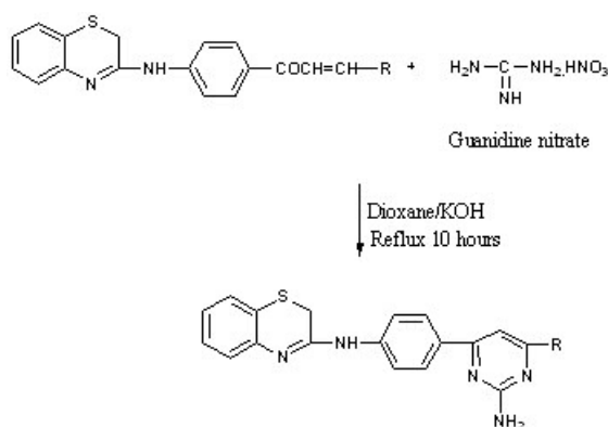
3[4'-(2"-Amino-4"- (substituted phenyl)-pyrimidine-4"-yl)-phenylamino] 1, 4-benzothiazines (5a-5d)
