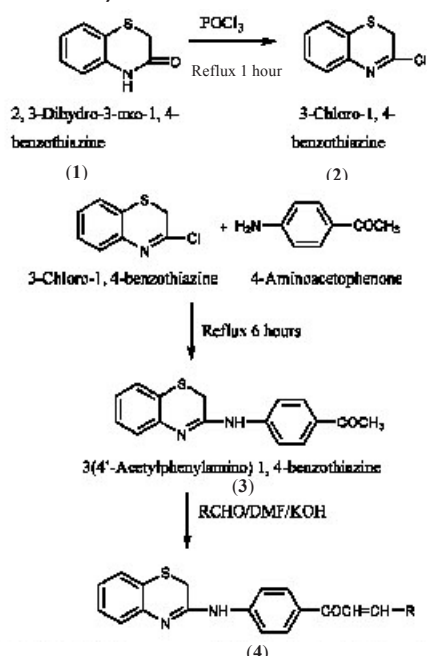
Scheme-1. Synthesis of substituted chalcones of 1, 4-benzothiazine from 2, 3-dihydro-3-oxo-1, 4-benzothiazines (4a-4j)
