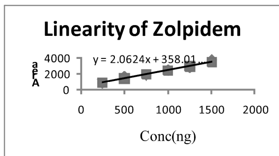
Fig.4: Linearity curve of ZOL at 254 nm
