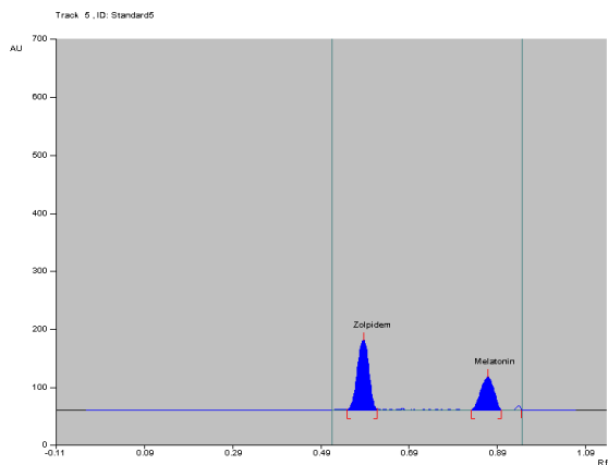
Fig. 2: HPTLC Chromatogram of standard MEL and ZOL in mixture
