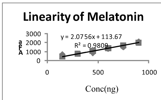
Fig.3: Linearity curve of MEL at 254 nm
