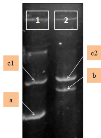
Fig. 1: Cleavage of supercoiled DNA by MJ protein: (lane 1): untreated pUC18, (lane 2): 6 µg of MJ protein. (a): The supercoiled DNA band, (b) linear DNA band, (c1 and c2): nicked circular DNA
