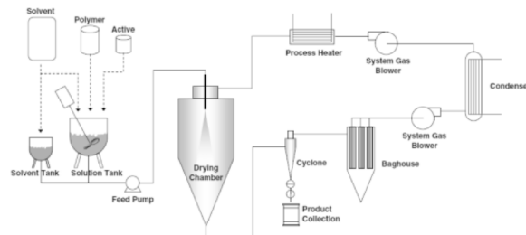
Fig. 6: Spray drying technique [Reproduced from: Rajput GC, Majmudar DF, Patel KJ, Patel NK, Thakor SR, Patel RR, et al. Floating drug delivery system- A review. Pharm. Ext. 2010; 1(1) 43-5.]
