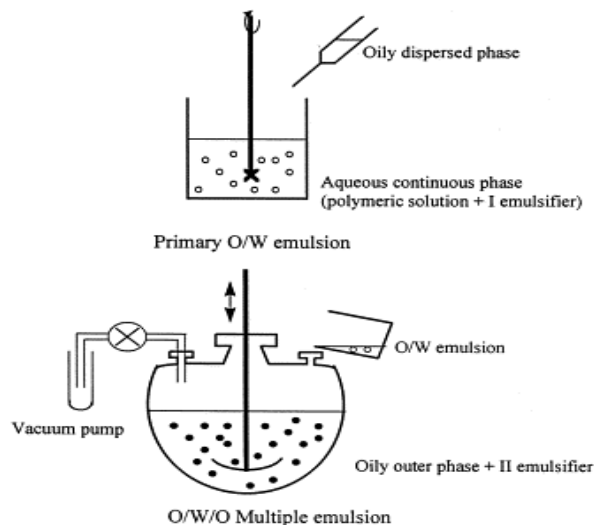
Fig. 5: Multiple Emulsion Method [Reproduced from: Patel G, Tiwari A, Rabadia N. Floating microspheres as a novel tool for H 2 receptor blocker. IRJP , 2012; 3(2): 45-52.]
