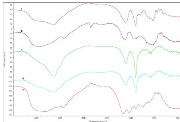
Figure 5. FT-IR spectra of (a) sodium alginate, (b) gum Arabic, (c) calcium alginate/gum Arabic without BSA, (d) alginate/gum Arabic containing BSA and (e) pure BSA.
