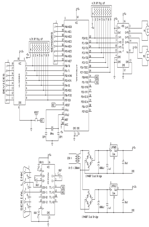
Fig.2. Circuit diagram
