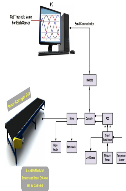
Fig.1. Block diagram of proposed work of the system
