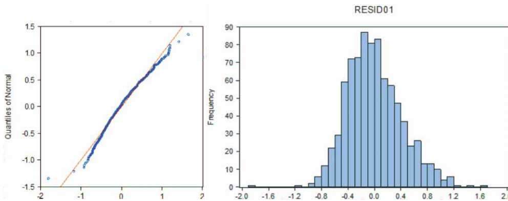
Figure 1: normal quintile graph of error term
