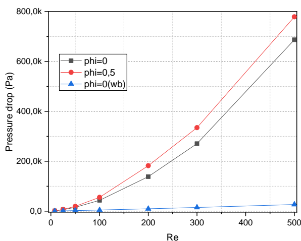
Figure .6: Evolution of the pressure drop with the different Reynolds number
