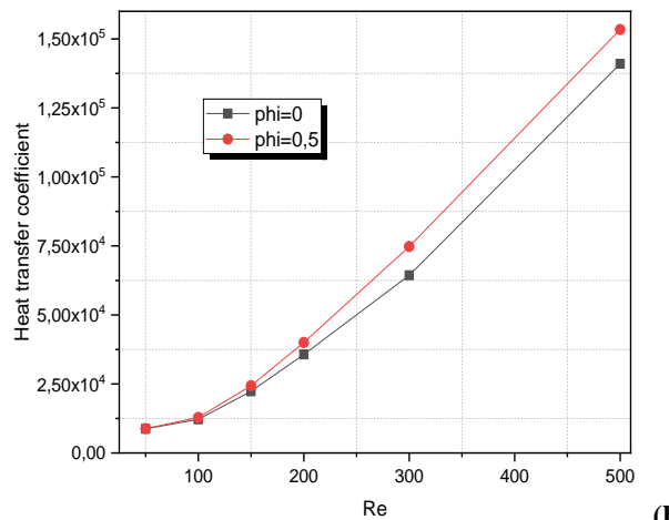
Figure .9: The evolution of Nu number (a) and Heat transfer coefficient (b) as a function of the Re with different values of ( \varphi )
