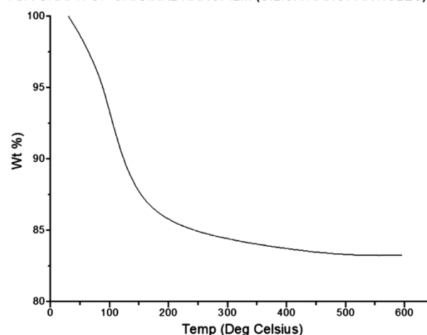
Fig. 7 — TGA Graph of the original Silica nanoparticles nanofilm
