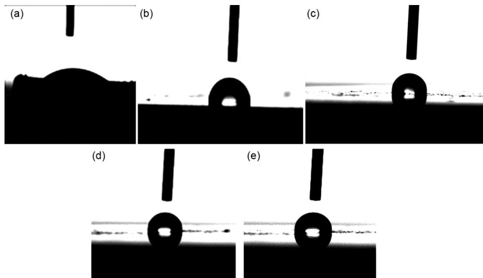
Fig. 6 — The WCA (water contact angle) of droplets of water on (a) the original glass surface, (b) HDTMS+0.3%Nano-SiO 2 , (c) HDTMS+0.6%Nano-SiO 2 , (d) HDTMS+2%Nano-SiO 2 , & (e) HDTMS+(3.6-4)%Nano-SiO 2 .
