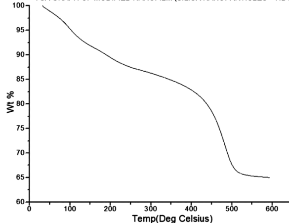
Fig. 8 — TGA Graph of the Modified Hydrophobic (0.6 % Silica nanoparticles + HDTMS) nanofilm.
