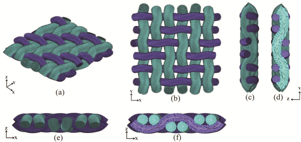
Fig. 7 — CAD of 2×2 twill weave fabrics with skewness property (a) isometric view, (b) top view (c) sideview, (d) cross-section at center line of yarn path for weft yarn, (e) front view, and (f) cross-section at center line of yarn path for warp yarn
