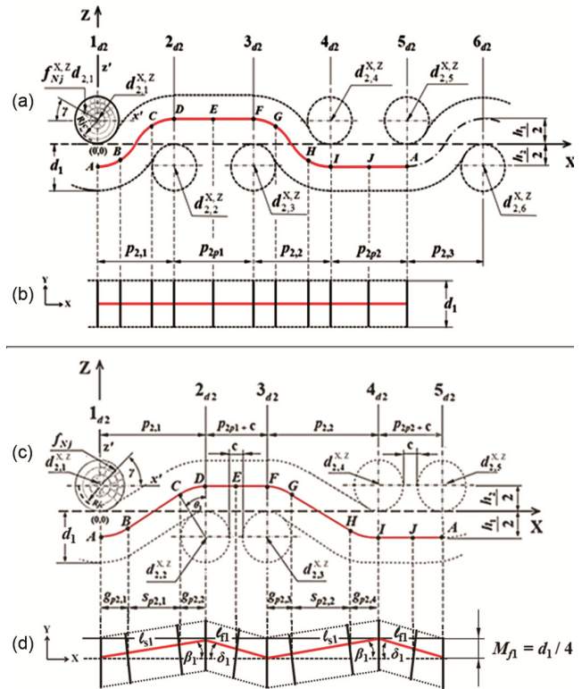
Fig. 2 — Coordinate system of filaments in 2x2 twill woven fabrics and the projection linear yarn path of floating and intersecting region [(a&b) the yarns are perpendicular to each other( \beta = 0 , \delta = 0 ) and (c&d) the inherent skewness of yarns]#
