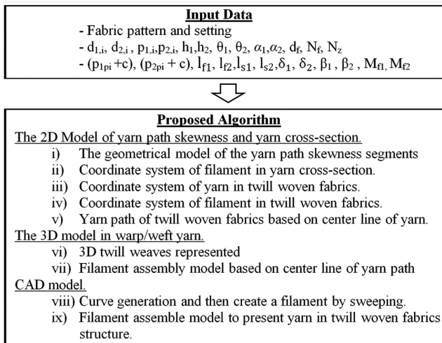
Fig. 1 — Major steps of computer modelling approach for constructing a 3D twill woven fabrics [ d_{1,i} , d_{2,i} = warp/weft yarn diameters; p_{1,i} , p_{2,i} = warp/weft yarn spacing at the crossover point; h_1 , h_2 = warp/weft crimp wave heights; \theta_1 , \theta_2 = warp/weft crimp angles; \alpha_1 , \alpha_2 = warp/weft yarn twist angle (degree); d_f = filament diameter; N_f = number of filament in yarn cross-section; and N_z = number of layer in yarn cross-section]
