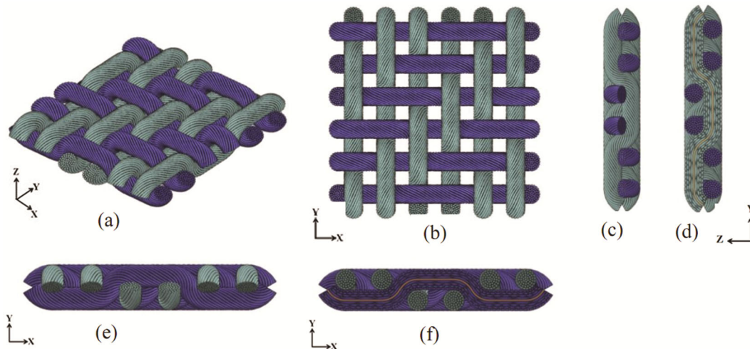
Fig. 5 — CAD of 2x2 twill weave fabrics (a) isometric view, (b) top view, (c) side view, (d) cross-section at center line of yarn path for weft yarn, (e) front view, and (f) cross-section at center line of yarn path for warp yarn 13
