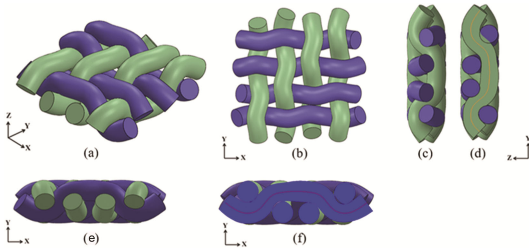
Fig. 4 — Thread model and 3D image of 2/2 twill fabrics structure with a single line of yarn path (a) isometric view, (b) top view, (c) side view, (d) cross-section at center line of yarn path for weft yarn, (e) front view, and (f) cross-section at center line of yarn path for warp yarn 2
