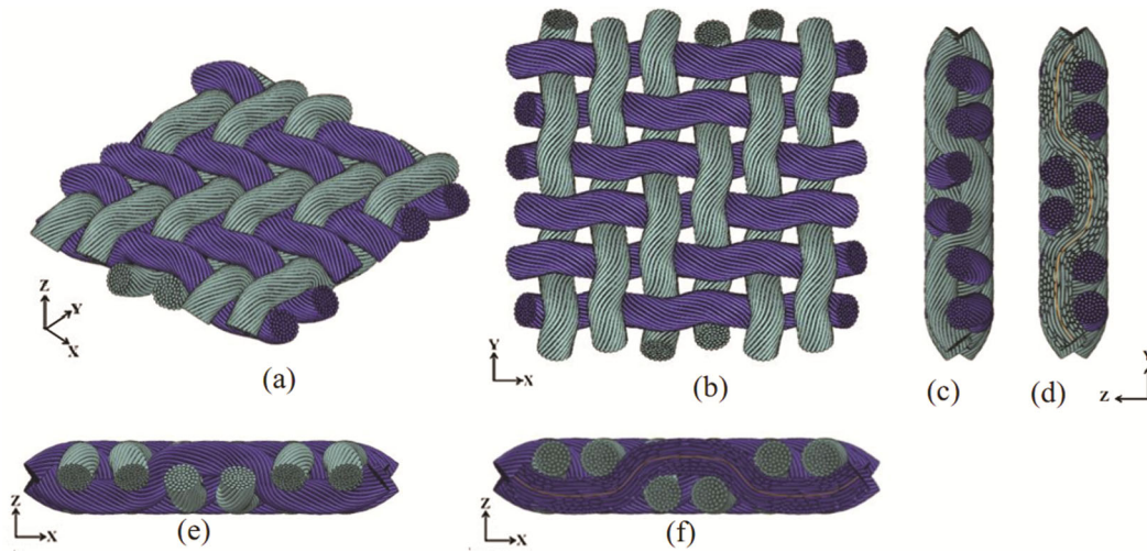
Fig. 6 — CAD of 2×2 twill weave fabrics with skewness property (a) isometric view, (b) top view, (c) side view, (d) cross-section at center line of yarn path for weft yarn, (e) front view, and (f) cross-section at center line of yarn path for warp yarn
