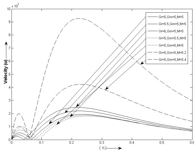
Fig 1: Effect of Gr, Gm and M on velocity profile when N=1, Pr=2 and t=1
