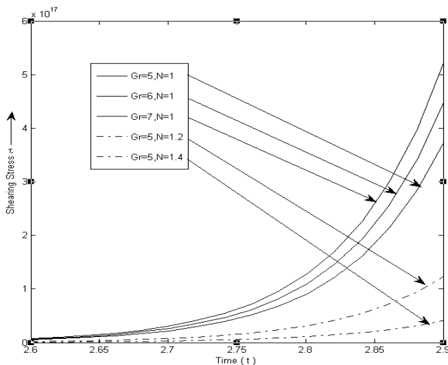
Fig 7: Effect of Gr and N on shearing stress when M=1 , Sc=2 , Pr=2 , Gm=5 , \epsilon = 0.02 and \omega=1
