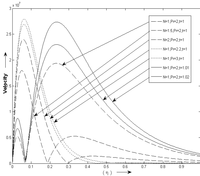
Fig 2: Effect of N, Pr and t on velocity profile when Gr=5, Gm=5 and M=5
