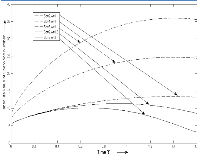
Fig 6: Effect of Sc and \omega on Sherwood Number when \epsilon = 0.02
