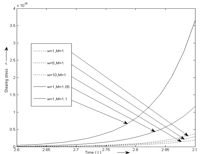
Fig 8: Effect of \omega and M on shearing stress when Gr=5 , Sc=2 , Pr=2 , Gm=5 , \epsilon = 0.02 and N=1
