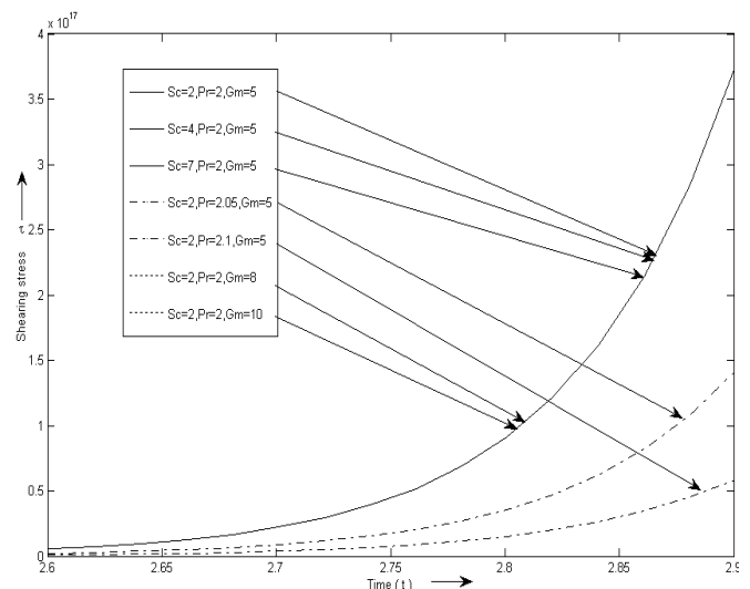
Fig 9: Effect of Sc , Pr and Gm on shearing stress when Gr=5 , \omega=1 , M=1 , \epsilon = 0.02 and N=1
