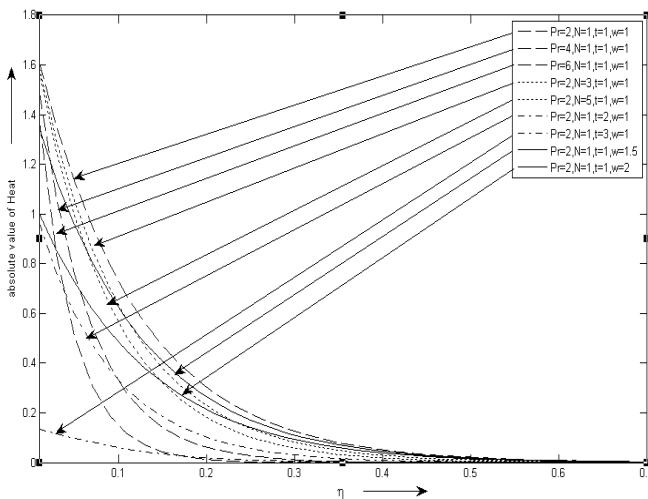
Fig 3: Effect of N, Pr, \omega and t on heat profile when \epsilon = 0.02
