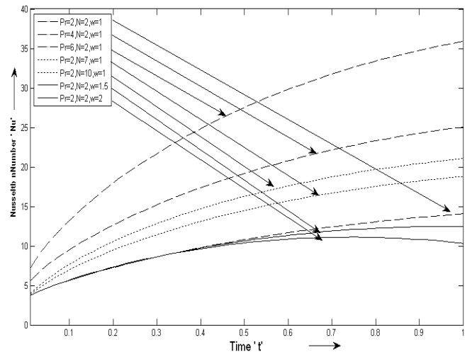
Fig 5: Effect of Pr, \omega and N on Nusselt Number when \epsilon = 0.02
