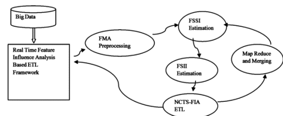
Fig. 1 — Architecture of proposed NCTS-FIA based ETL framework
