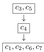
Figure 1. Diagram of Partition P_{e_2,0.69}^\tau
