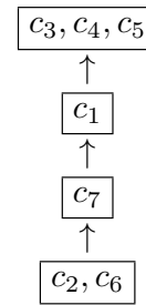
Figure 2. Diagram of Partition P_{e_2,0.31}^\tau
