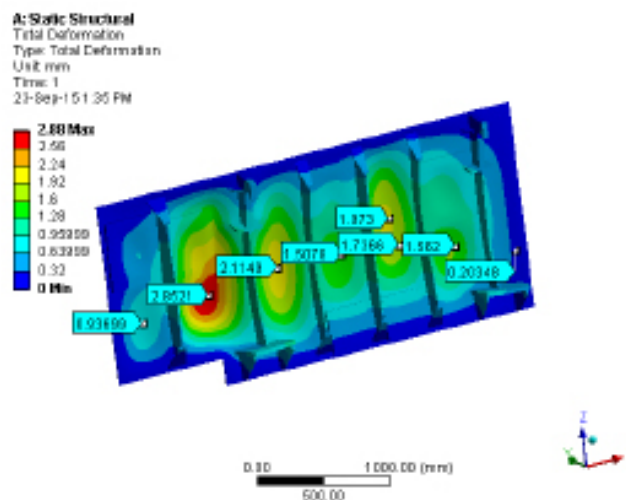
Figure 4. Result Plot (Individual wall)
