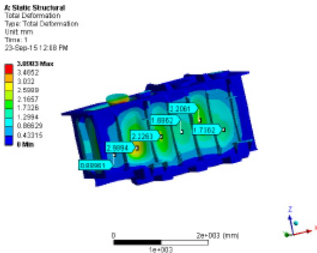
Figure 3. Result Plot (Tank)
