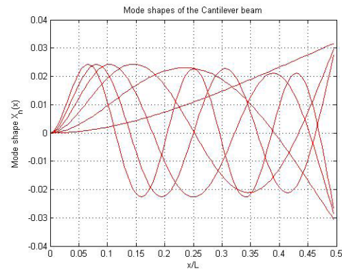
Figure 1. Mode shape of first six modes.
