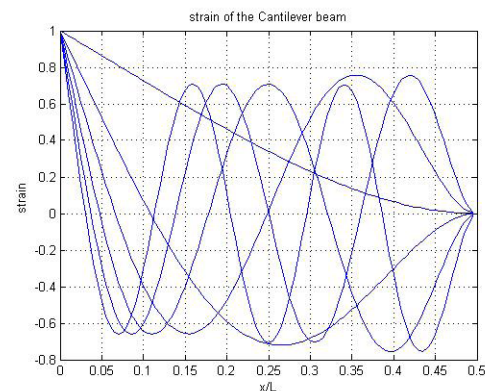
Figure 2. Strain shape of first six modes.
