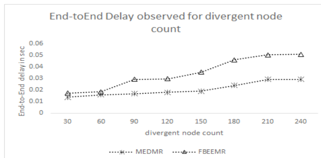
Figure 4. End-to-end delay observed for divergent node count
