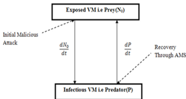
Figure 2. Predator-Prey Model for cloud based Network
