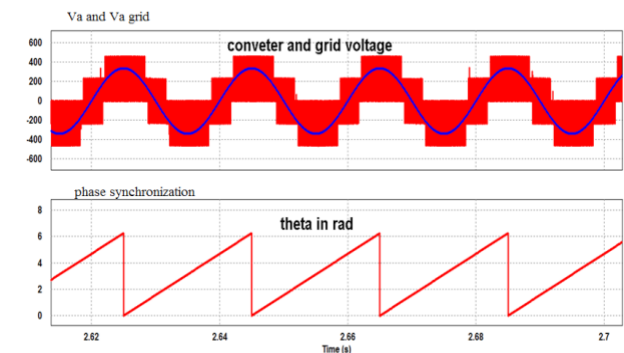
Figure 6. Grid synchronization.
