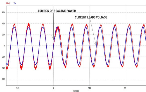
Figure 10. Addition of reactive power.
