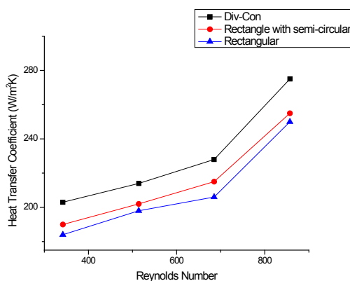
Figure 5. Reynolds Number vs. heat transfer coefficient at 75 W.
