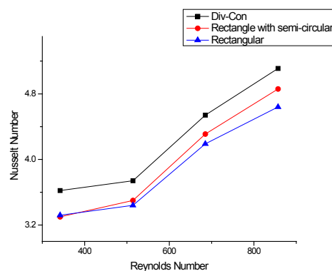
Figure 8. Reynolds Number vs. Nusselt Number at 50 W.
