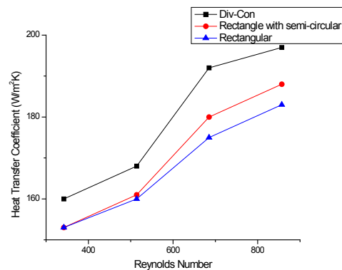
Figure 7. Reynolds Number vs. heat transfer coefficient at 125 W.
