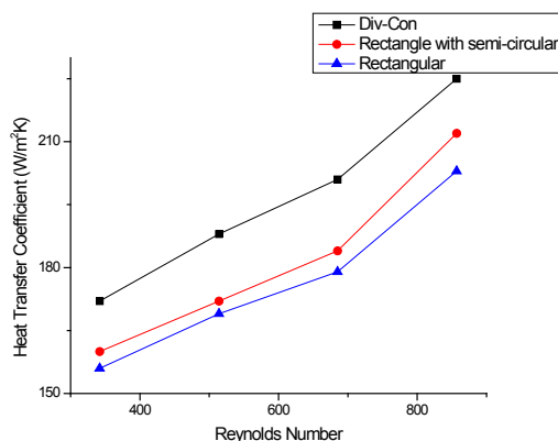
Figure 6. Reynolds Number vs. heat transfer coefficient at 100 W.
