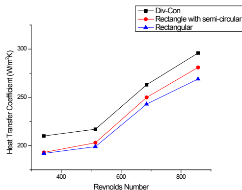
Figure 4. Reynolds Number vs. heat transfer coefficient at 50 W.
