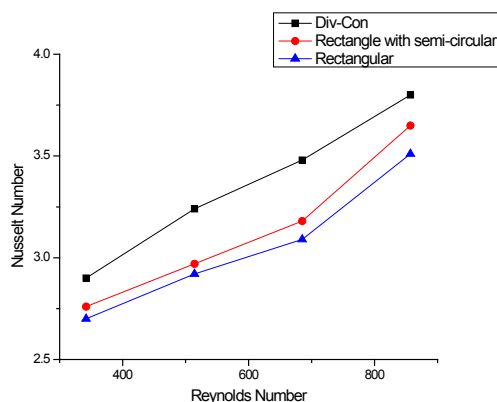
Figure 10. Reynolds Number vs. Nusselt Number at 100 W.
