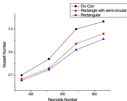
Figure 11. Reynolds Number vs. Nusselt Number at 125 W.
