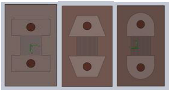
Figure 3. Assembly with rectangular, divergent-convergent and rectangle with semi-circular manifold arrangements.
