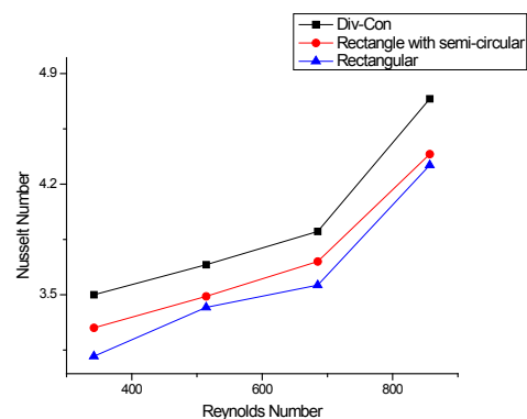
Figure 9. Reynolds Number vs. Nusselt Number at 75 W.
