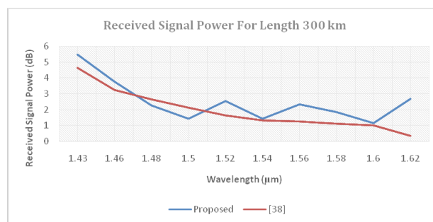
Figure 8. Received Signal Power for Length 300 km.
