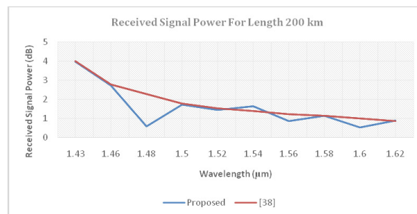
Figure 7. Received Signal Power for Length 200 km.
