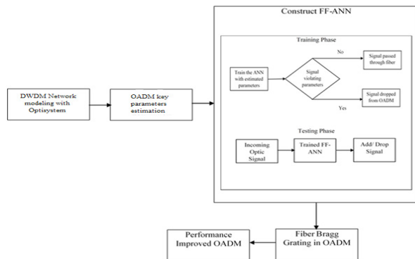
Figure 1. Functional Block diagram of the proposed method.
