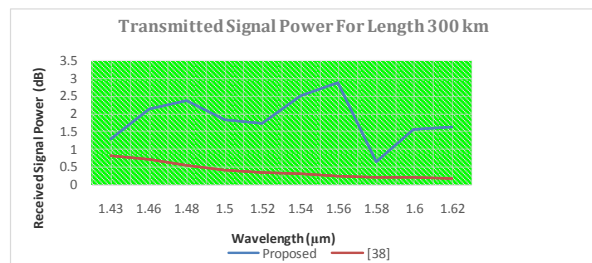
Figure 6. Transmitted Signal Power for Length 300 km.
