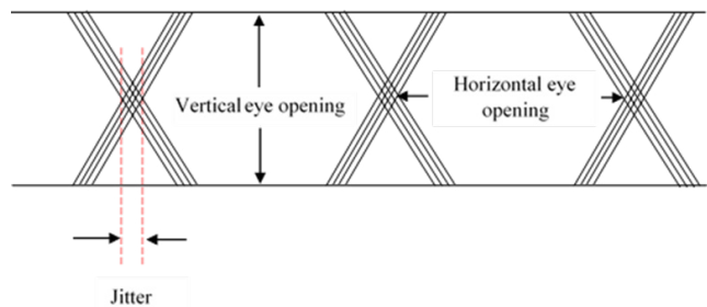
Figure 2. Jitter measured from the eye diagram of the system.
