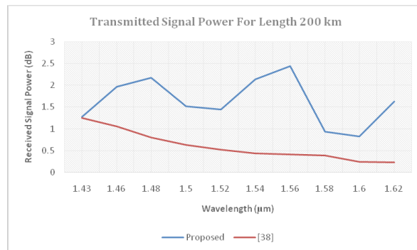
Figure 5. Transmitted Signal Power for Length 200 km.
