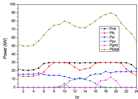
Figure 4. Generation scheduling results obtained using MAIMD-Model 2.
