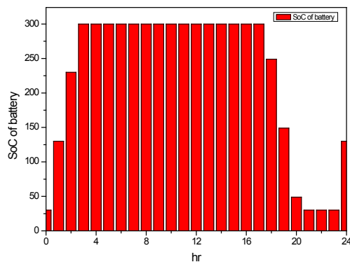
Figure 10. State of charge of the battery.
