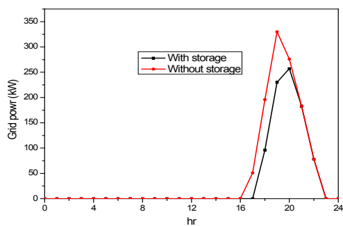
Figure 7. Power drawn from grid.
