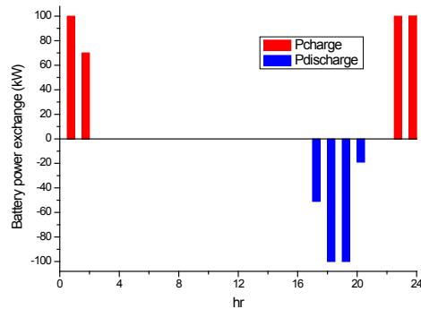
Figure 9. Battery power exchange.
