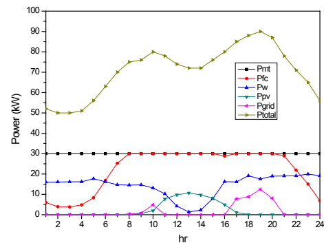
Figure 3. Generation scheduling results obtained MAIMD-Model1 algorithm.
