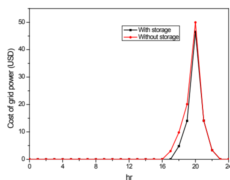
Figure 8. Cost of power drawn from grid.
