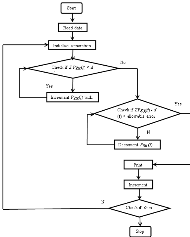
Figure 1. Flow chart of MAIMD algorithm.
