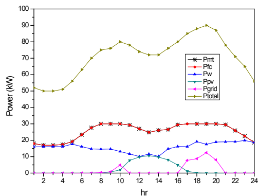
Figure 2. Generation scheduling results obtained using AIMD algorithm.
