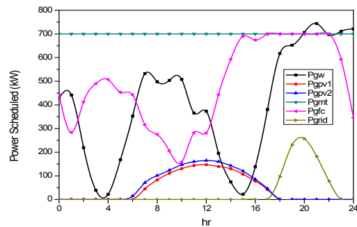
Figure 6. Generation scheduling with storage.
