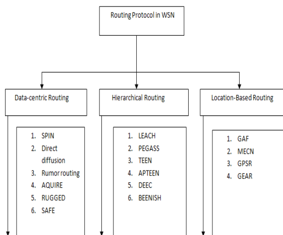
Figure 1. Routing protocol in WSN.
