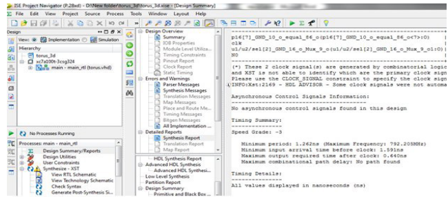
Figure 9. Timing report.
