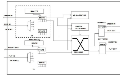
Figure 1. 2D router design.
