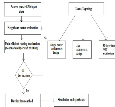
Figure 6. Proposed flow.
