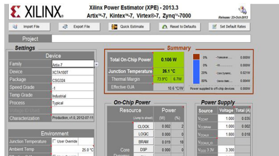
Figure 8. Power utilization.
