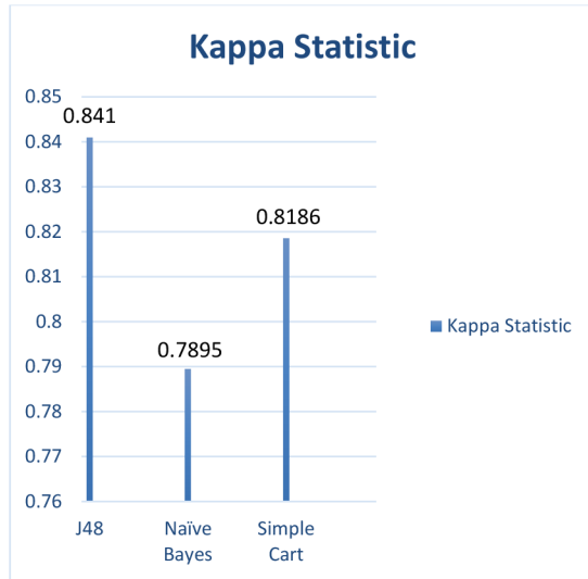
Figure 3. Kappa statistics of J48, Naive Bayes and Simple Cart.
