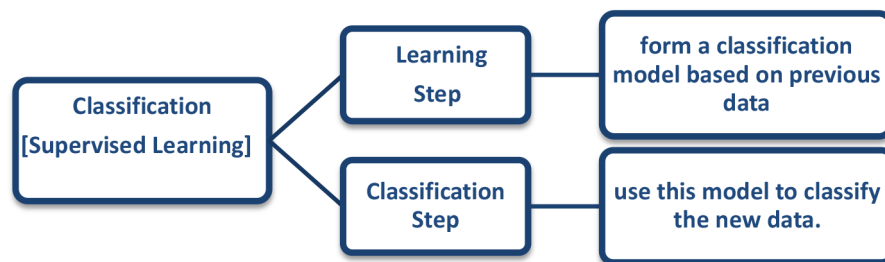
Figure 1. Classification technique.
