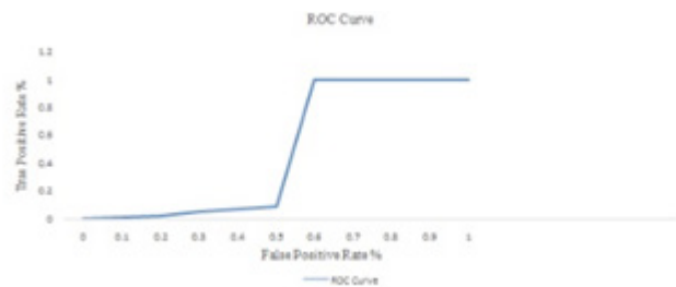
Figure 4. ROC curve.
