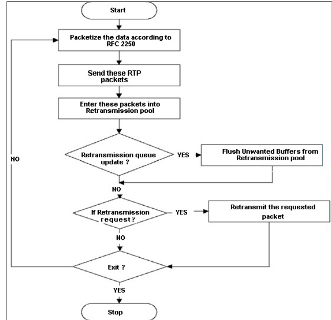
Figure 7. Flow chart: buffer under-flow – pseudocode.
