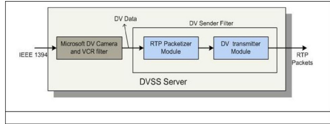
Figure 3. DV server functional block diagram.
