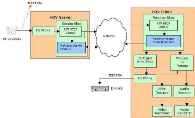
Figure 4. HDV server components.
