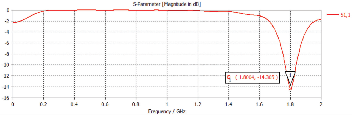
Figure 6. The Simulated plot for S_{11} Parameter 2 .
