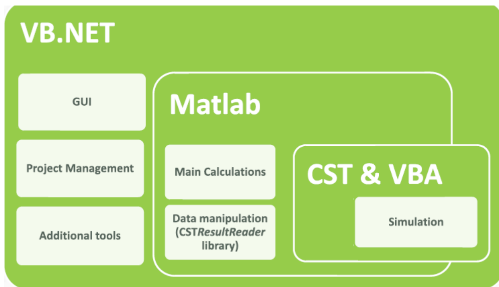
Figure 3. VBA Interfacing Architecture 11 .
