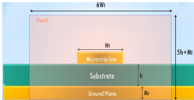
Figure 2. Side view of microstrip patch antenna 8 .
