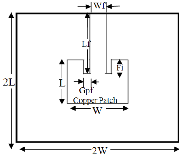
Figure 1. Top view of inset microstrip patch antenna 8 .
