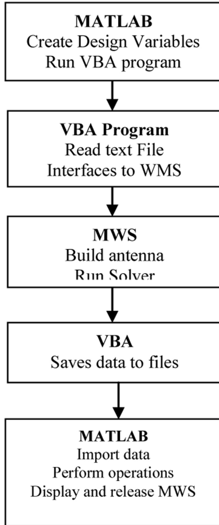
Figure 5. Flow chart for MATLAB-CST Interfacing 11 .
