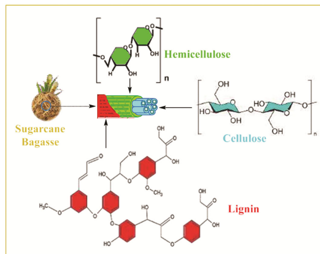
Fig. 1 — Structure of lignocellulosic biomass with cellulose, hemicellulose and lignin
